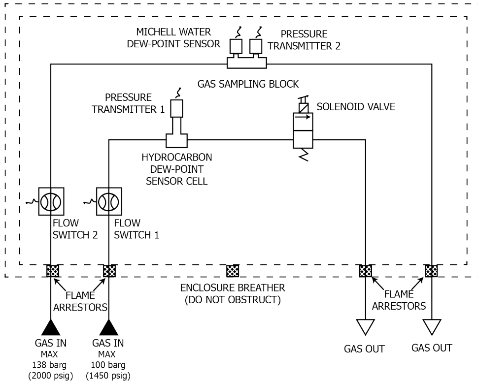
Figure 4 Flow Schematic
